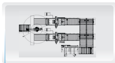
C CNC - one to two machines with manipulator
