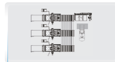
C CNC - one to three connection line
